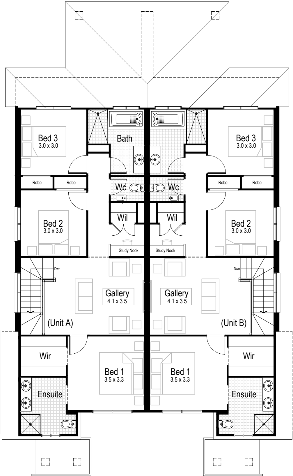
First Floor
